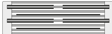
Extended double side metallized carrier film design with internal series connection and metallized film (series connection of 2 elements)
