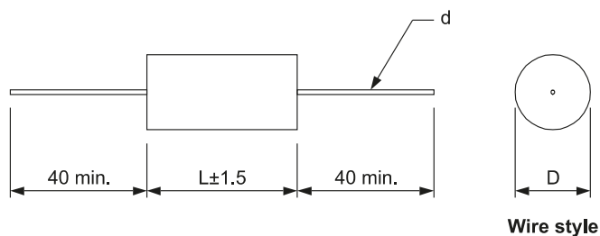
MPH wire terminals style article table (different values available upon request)
