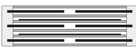
Extended foil design with internal series connection and metallized film (series connection of 2 elements)
